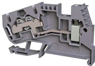
Screw spring clip with inscription 2x4 labels
