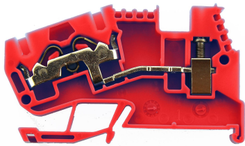
Screw spring clip with inscription 2x4 labels
