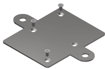
Retaining plate for junction box 48953/48955
